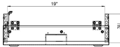
Front View Without Door
